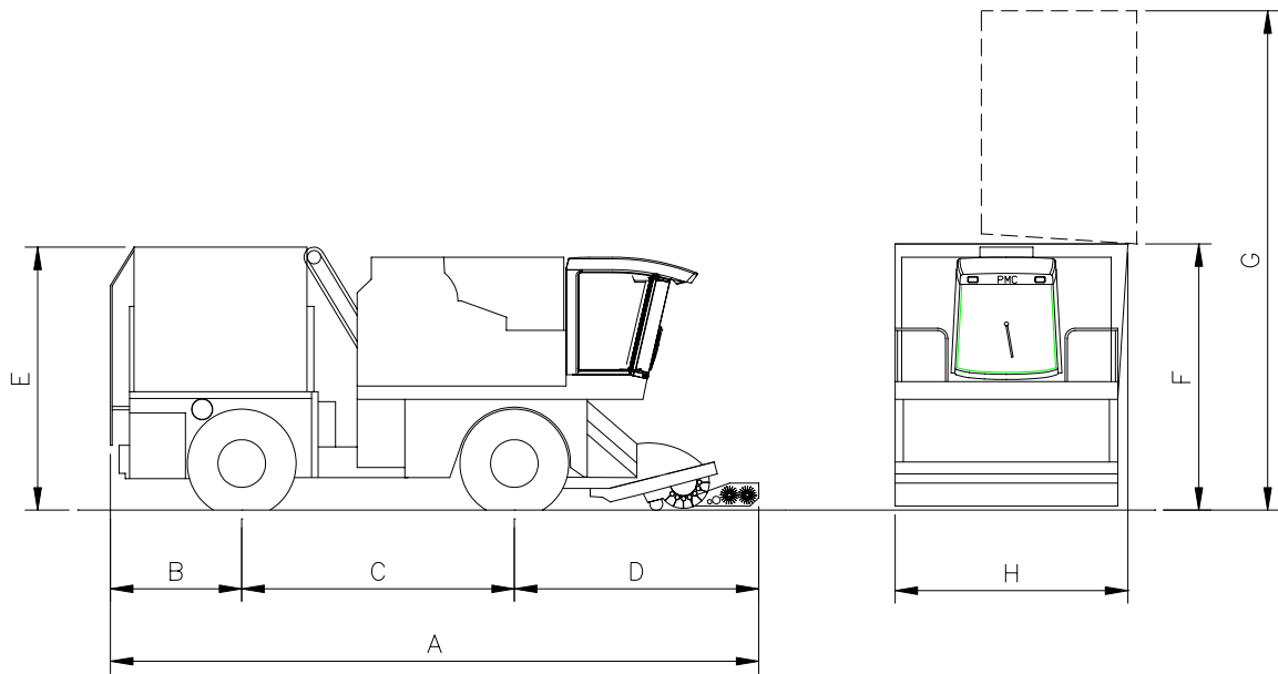
Side & Front elevation of machine
